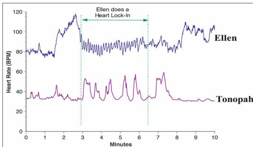
Figure 6.12. Heart-rhythm patterns of woman and horse.
